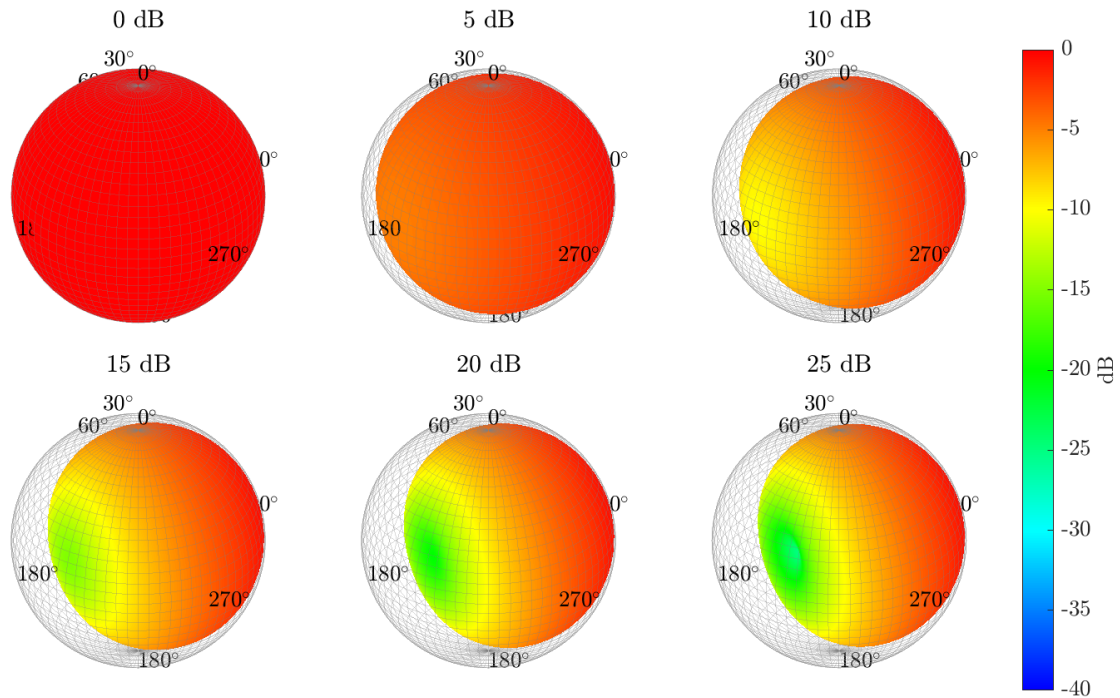
Figure 3: Normalized shading function W_L for various levels of attenuation L .
