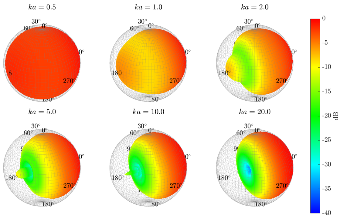
Figure 5: Normalized balloons of the shading function W_s for a point source on a sphere at (\theta_0, \phi_0) = (\pi/2, 0) and various ka values. Diffraction spots and generally increasing attenuation appear behind the sphere with increasing frequency.
