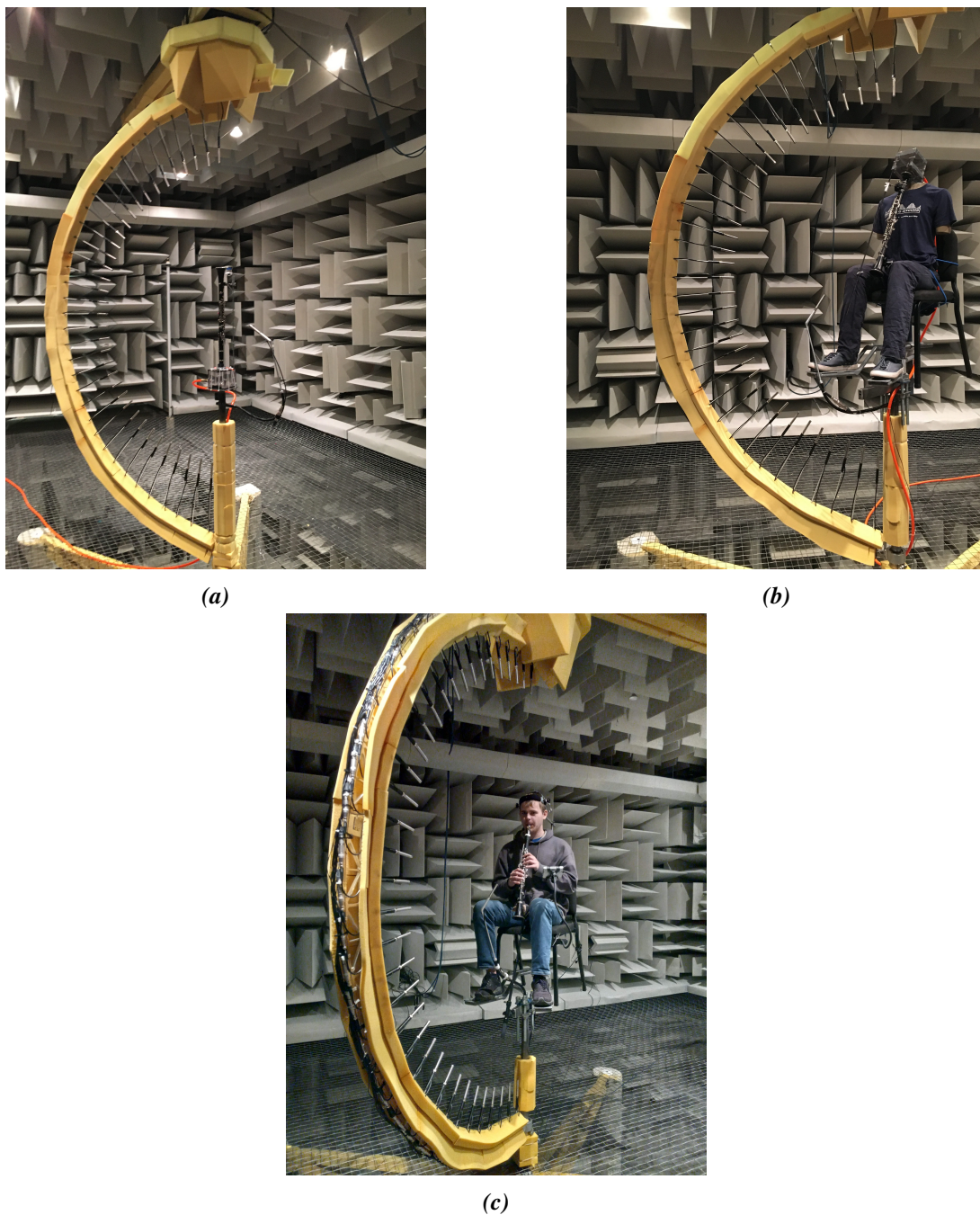
Figure 6: Three clarinet directivity measurement setups. (a) Isolated clarinet with blowing apparatus, oriented upside down. (b) Clarinet and blowing apparatus attached to a mannequin in playing position, with the blowing apparatus replacing the mannequin head. (c) Naturally played clarinet with a clarinetist.
